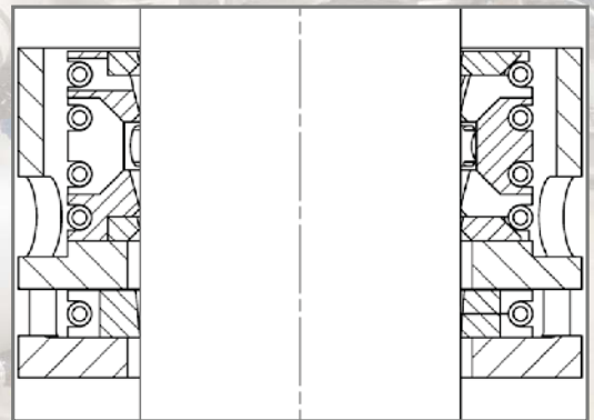
New concept BOSS, fitting into the standard case
