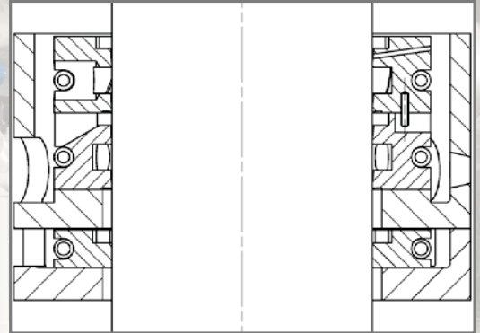
Standard oil wiper packing
